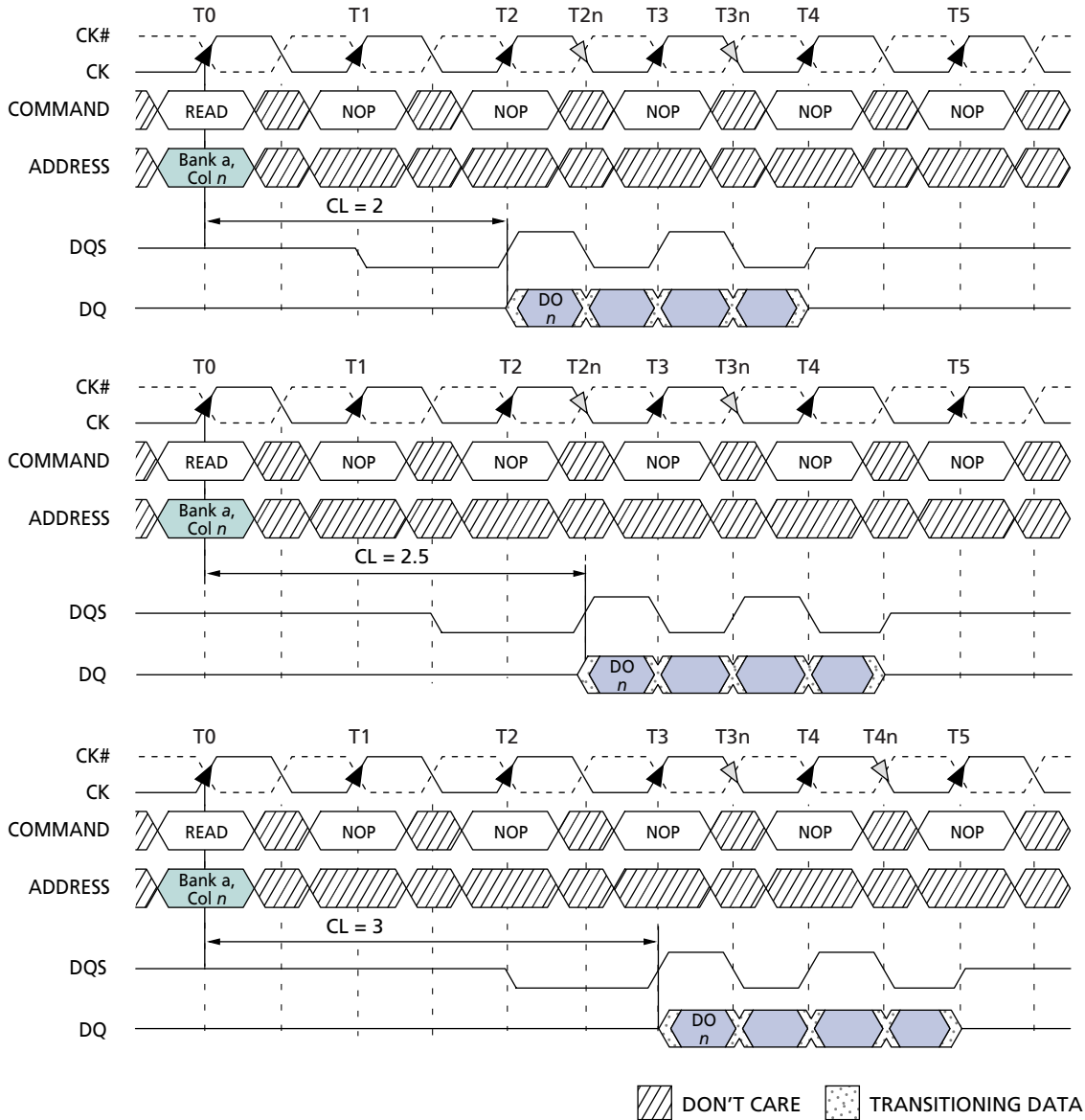
Figure 13: READ Burst
