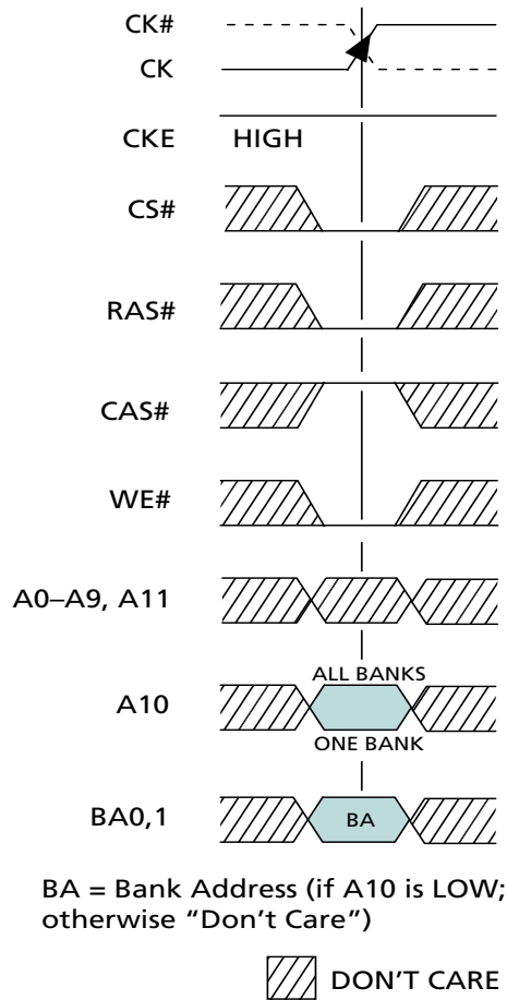
Figure 31: PRECHARGE Command
