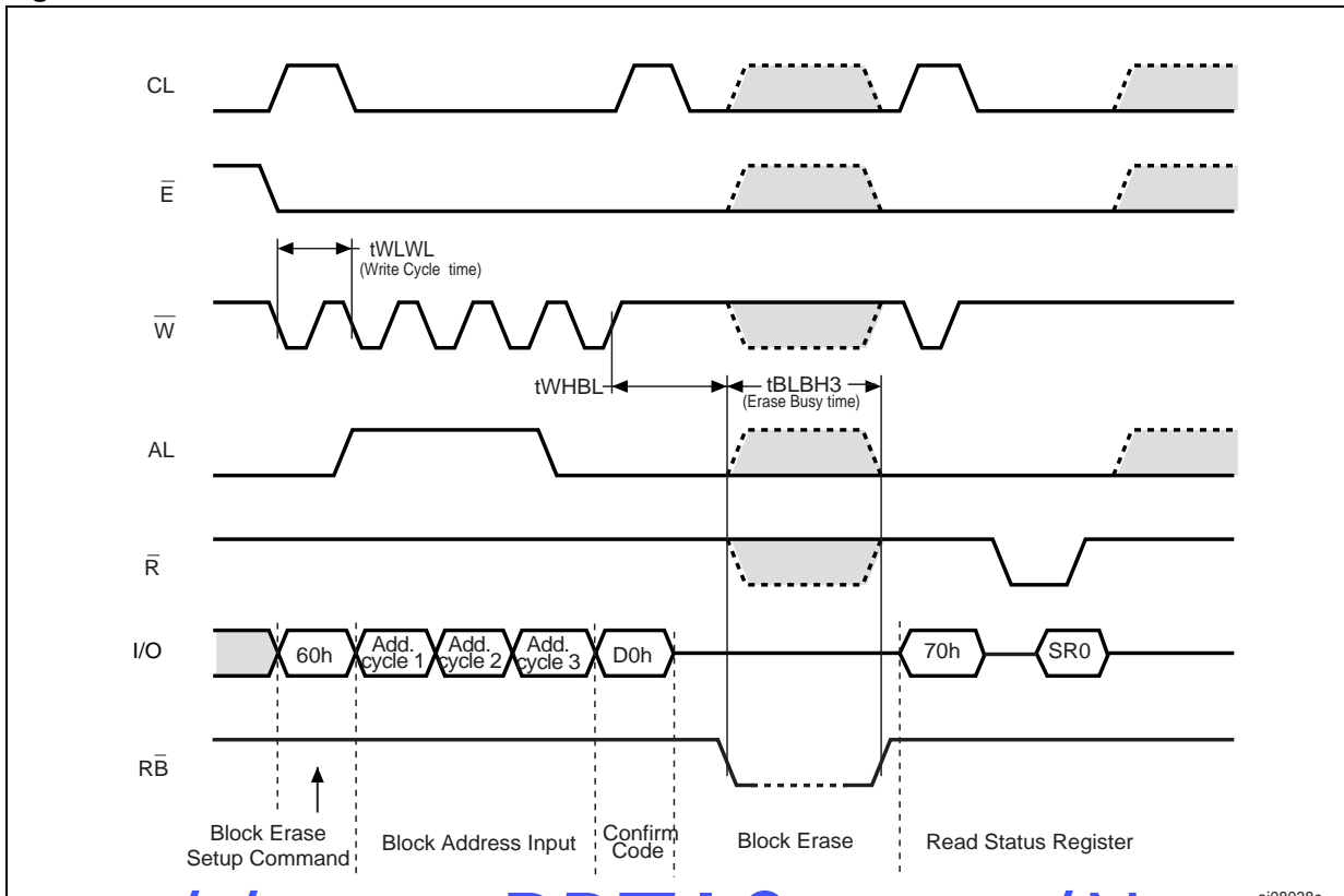
Figure 21. Block Erase AC Waveform
