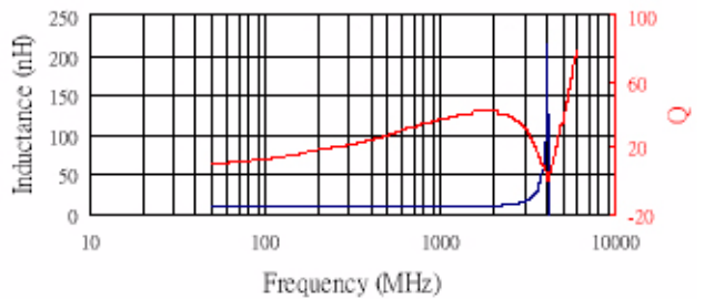
AL03GT12N
