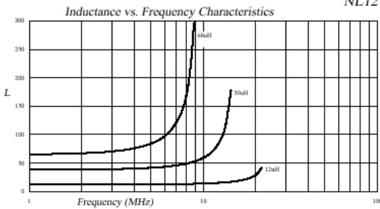
NL12 Series
