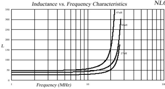
NL10 Series
