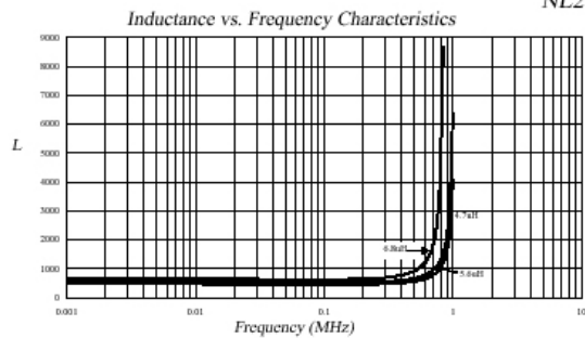
NL20 Series
