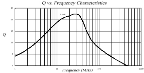
NL05 series
