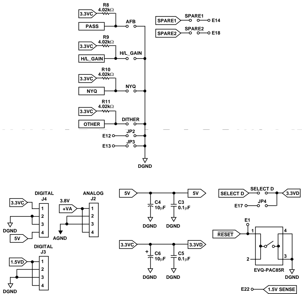
Figure 24. Evaluation Board
