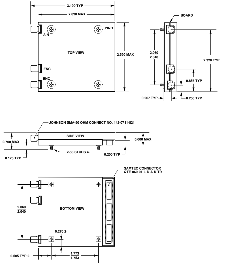
Figure 39. Non-Hermetic Hybrid—Surface-Mounted Parts (WS-Suffix)
