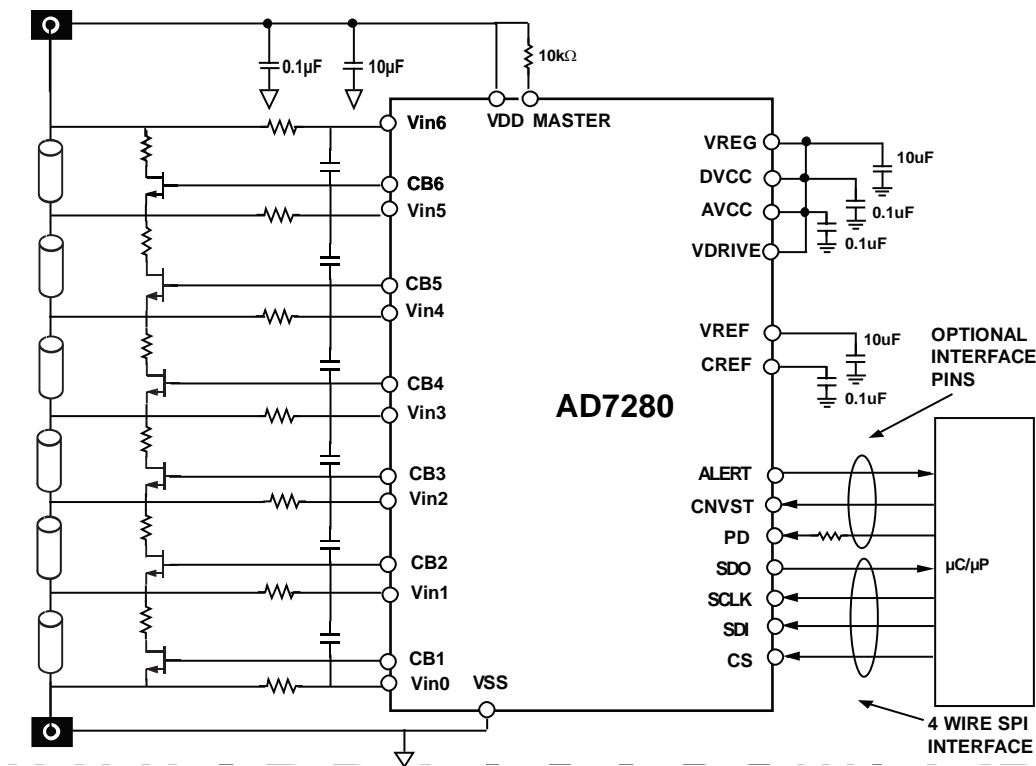
Figure 10. AD7280 Configuration Diagram for 6 Battery Cells
