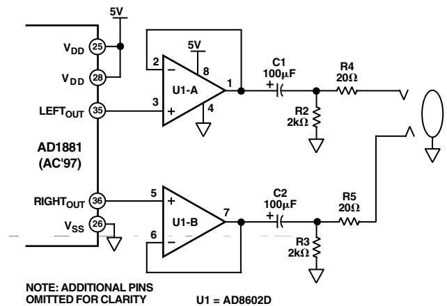
Figure 8. A PC100 Compliant Line Output Amplifier
