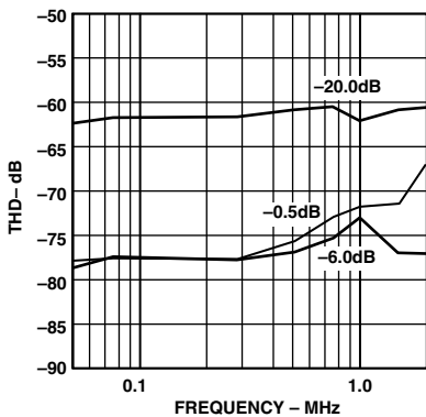
TPC 7. THD vs. Input Frequency (Input Span = 5.0 V p-p, V CM = 2.5 V)
