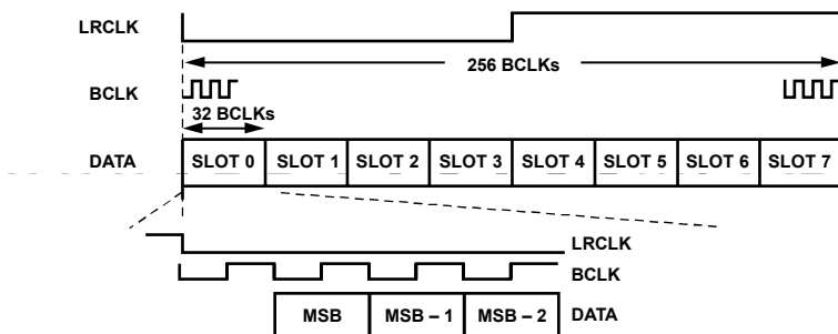
Figure 34. 8-Channel TDM Mode with Clock
