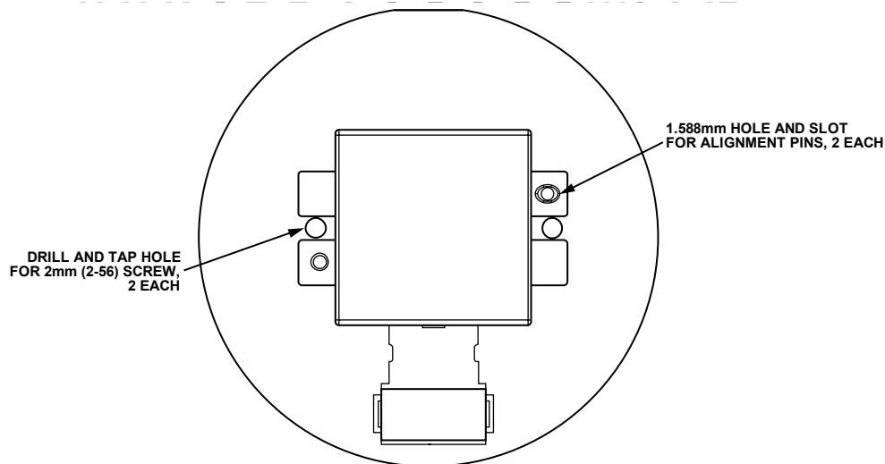
Figure 33. Mechanical Attachment
