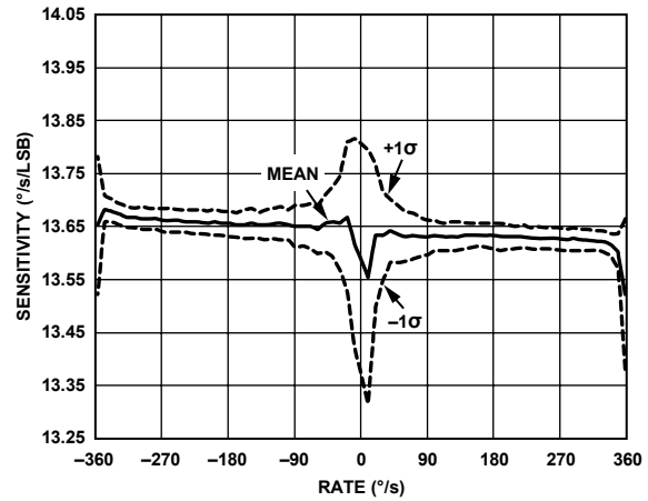
Figure 20. Gyroscope Linearity
