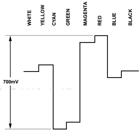
Figure 120. Pr Levels—PAL
