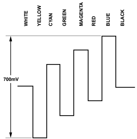
Figure 121. Pb Levels—PAL
