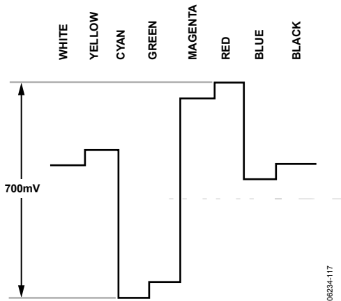
Figure 117. Pr Levels—NTSC
