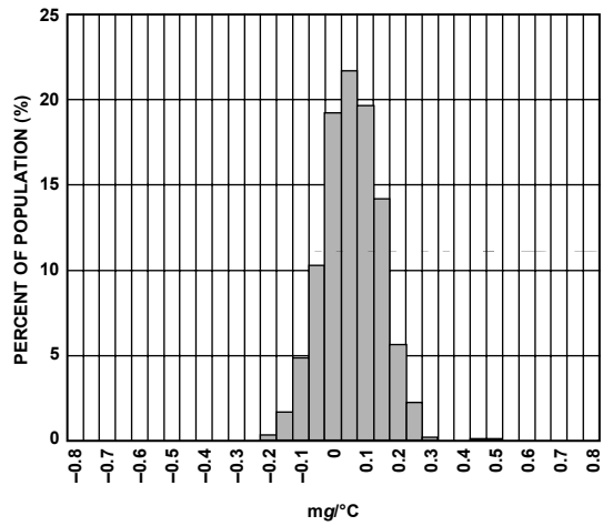
Figure 5. X-Axis Zero g Bias Temperature Coefficient
