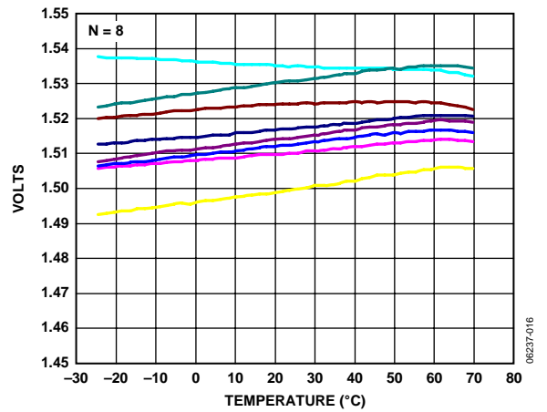
Figure 16. Y-Axis Zero g Bias vs. Temperature; Eight Parts Soldered to PCB, V_5 = 3\text{ V}
