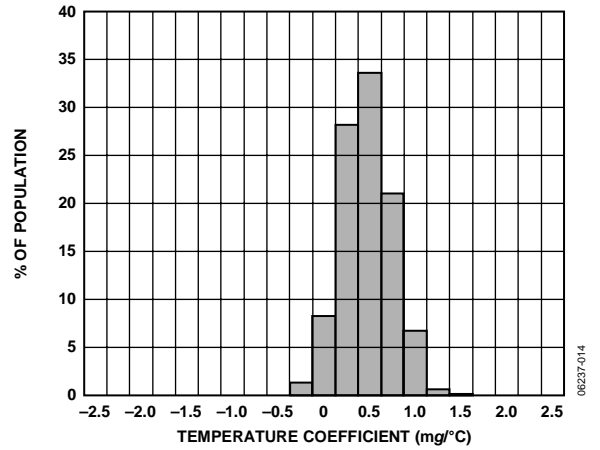
Figure 14. Y-Axis Zero g Bias Temperature Coefficient, V_5 = 3\text{ V}
