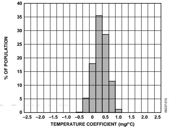
Figure 15. Y-Axis Zero g Bias Temperature Coefficient, V_5 = 5\text{ V}
