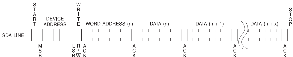
Figure 1. Page Write
