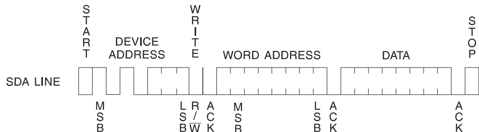
Figure 8-2. Byte Write
