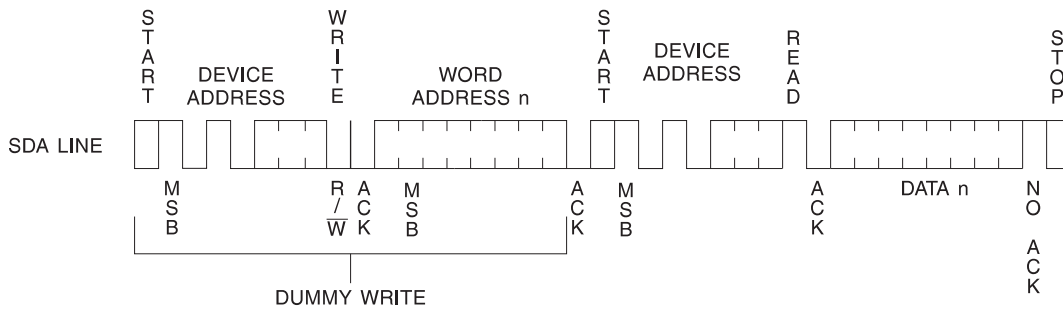
Figure 14. Random Read
