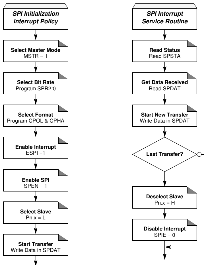
Figure 19-10. Master SPI Interrupt Policy Flows
