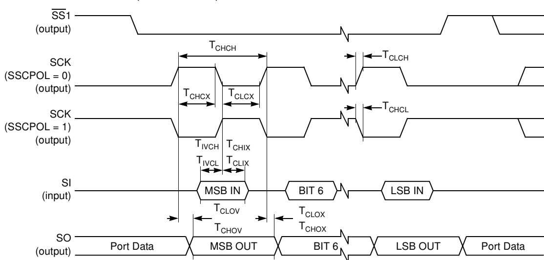
Figure 23-15. SPI Master Waveforms (SSCPHA = 1)
