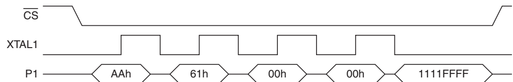
Figure 23-18. Read User Fuses Sequence
