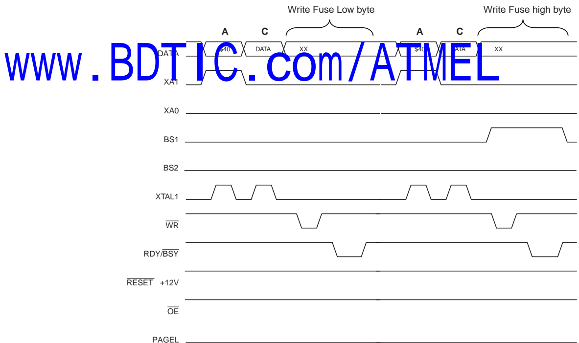
Figure 131. 熔丝位编程波形
