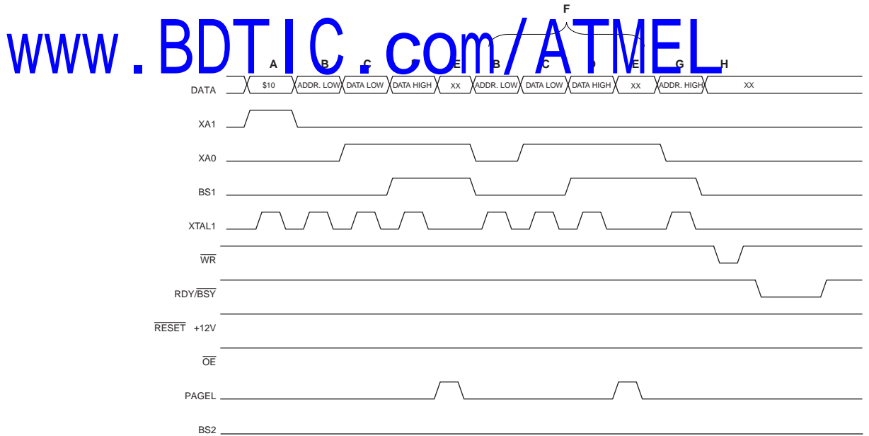
Figure 129. Flash 编程波形 (1)
