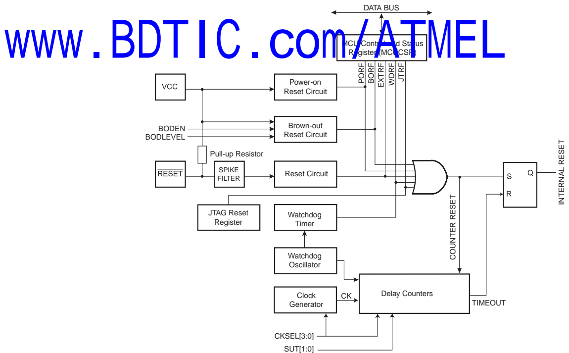
Figure 15. 复位逻辑
