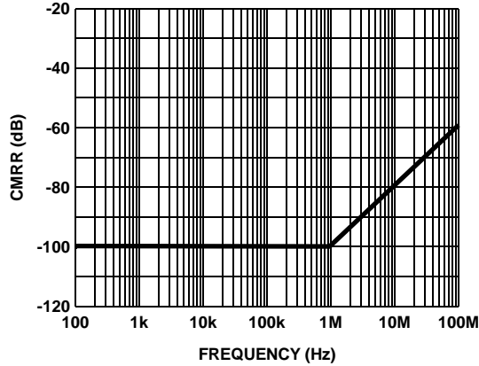
FIGURE 23. CMRR
