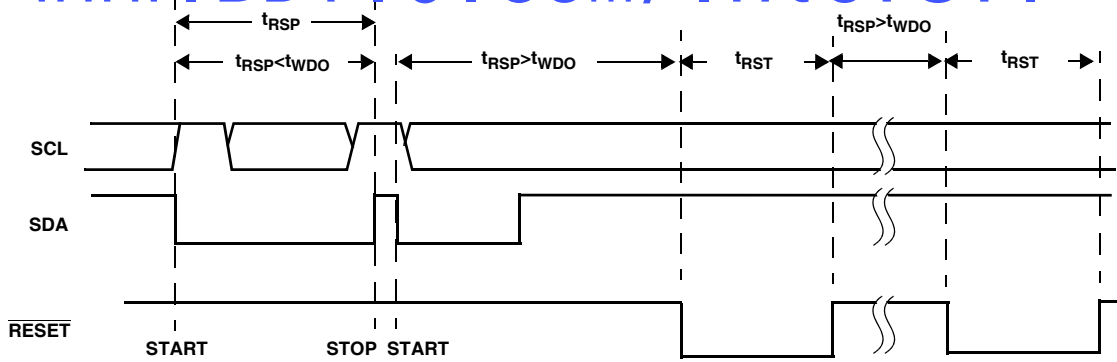
FIGURE 3. WATCHDOG TIMING
