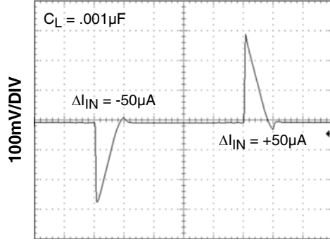
50µA LOAD TRANSIENT RESPONSE
