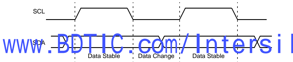
FIGURE 14. VALID DATA CHANGES ON THE SDA BUS
