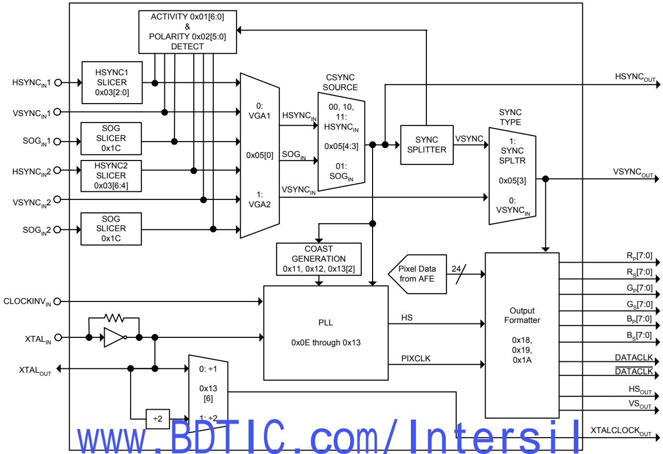
FIGURE 8. SYNC FLOW
