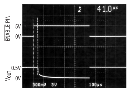
\overline{ENABLE} Pin Response Time
