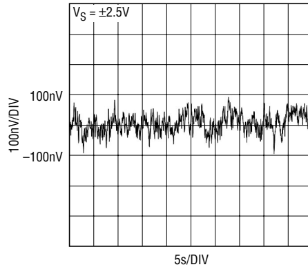
0.1Hz to 10Hz Output Voltage Noise
