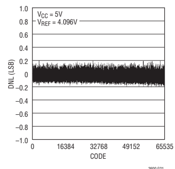
Differential Nonlinearity (LTC2600)
