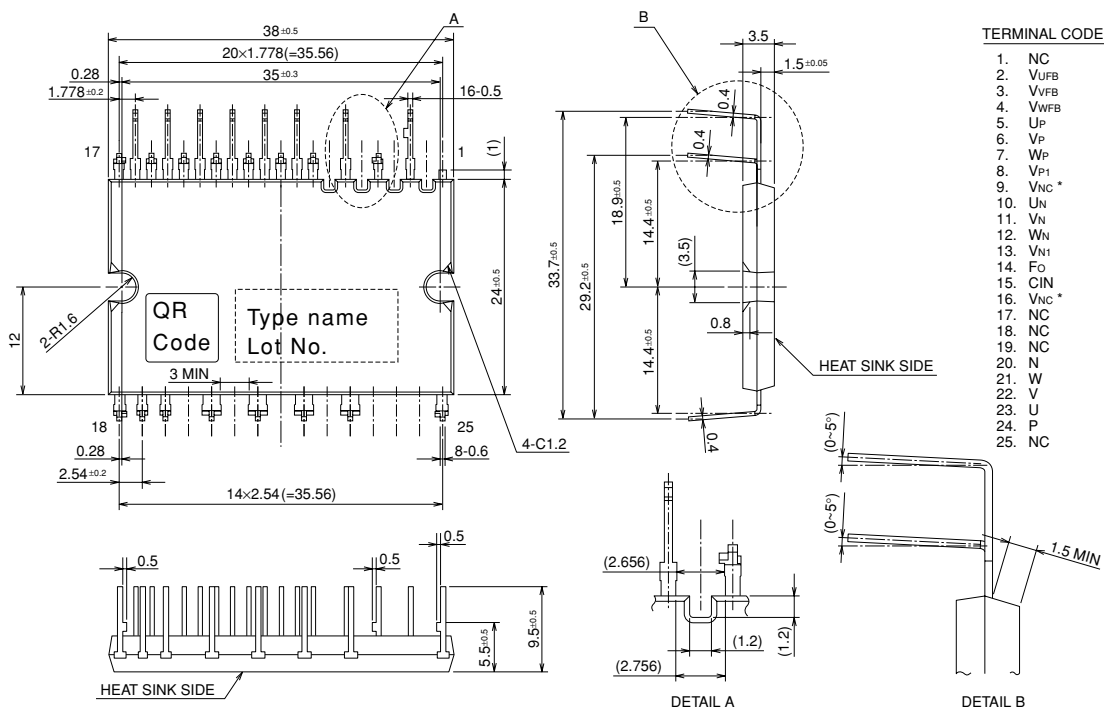
Fig. 3 ZIGZAG TERMINAL TYPE PACKAGE OUTLINES (PS21961-4C)
