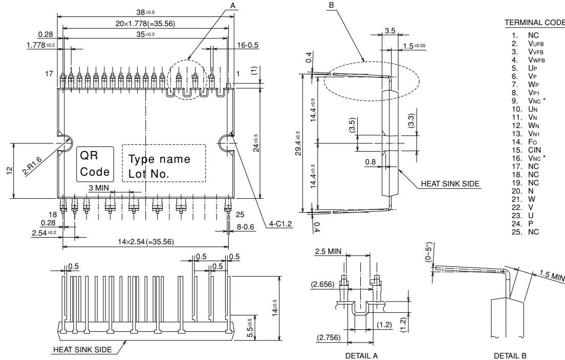
Fig. 2 LONG TERMINAL TYPE PACKAGE OUTLINES (PS21961-4A)
