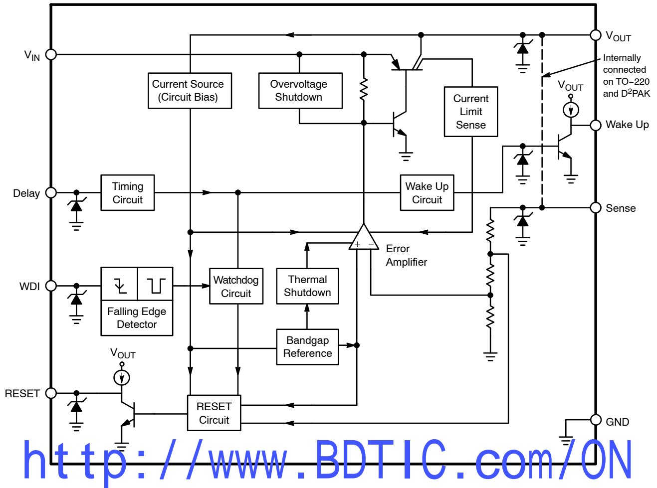
Figure 1. Block Diagram
