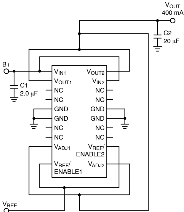
Figure 13. 400 mA Loading
