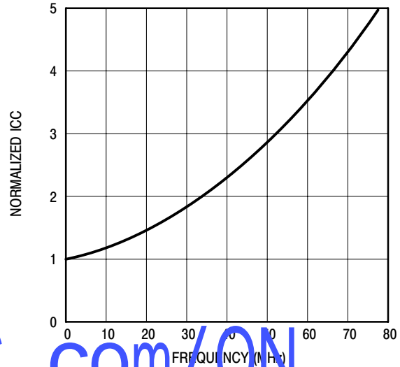
Figure 1. I_{CC} versus Frequency (No Load)
