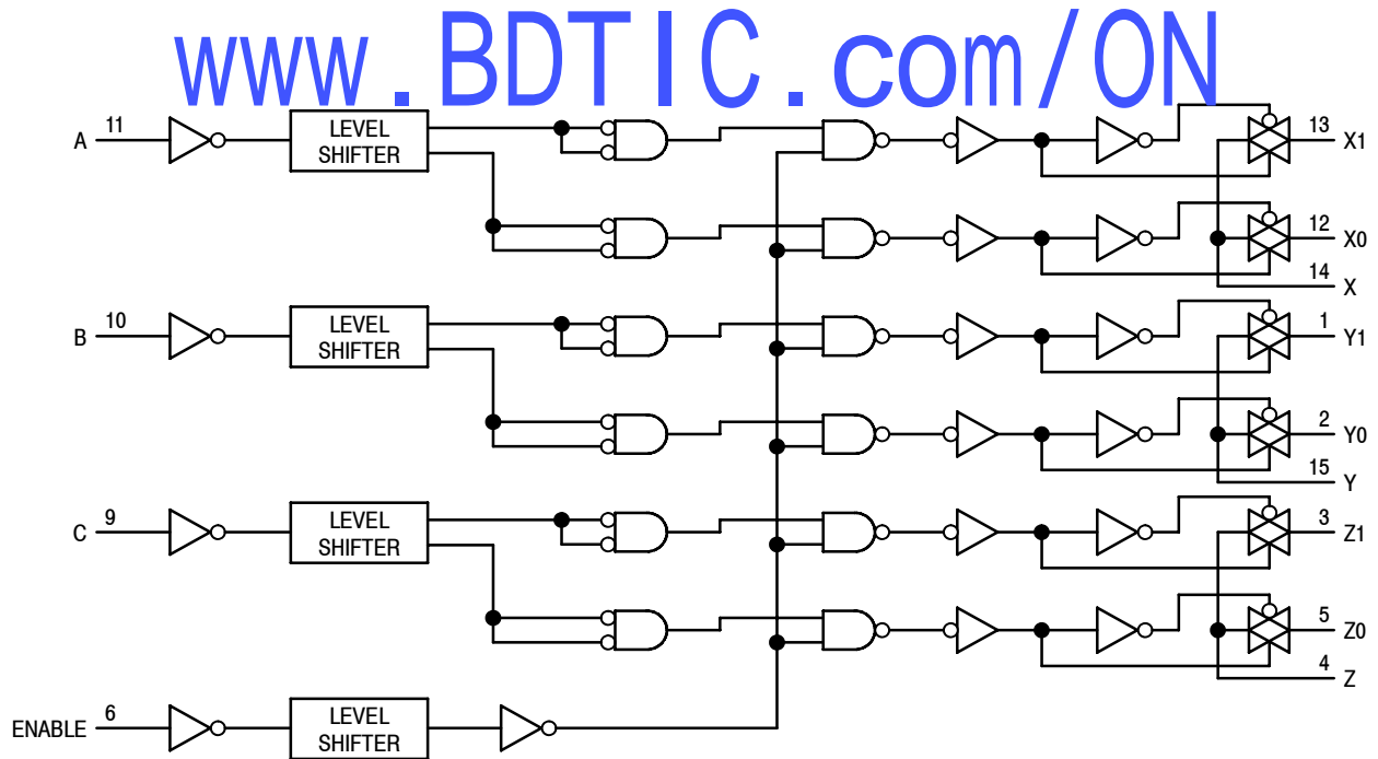
Figure 32. Function Diagram, VHC4053
