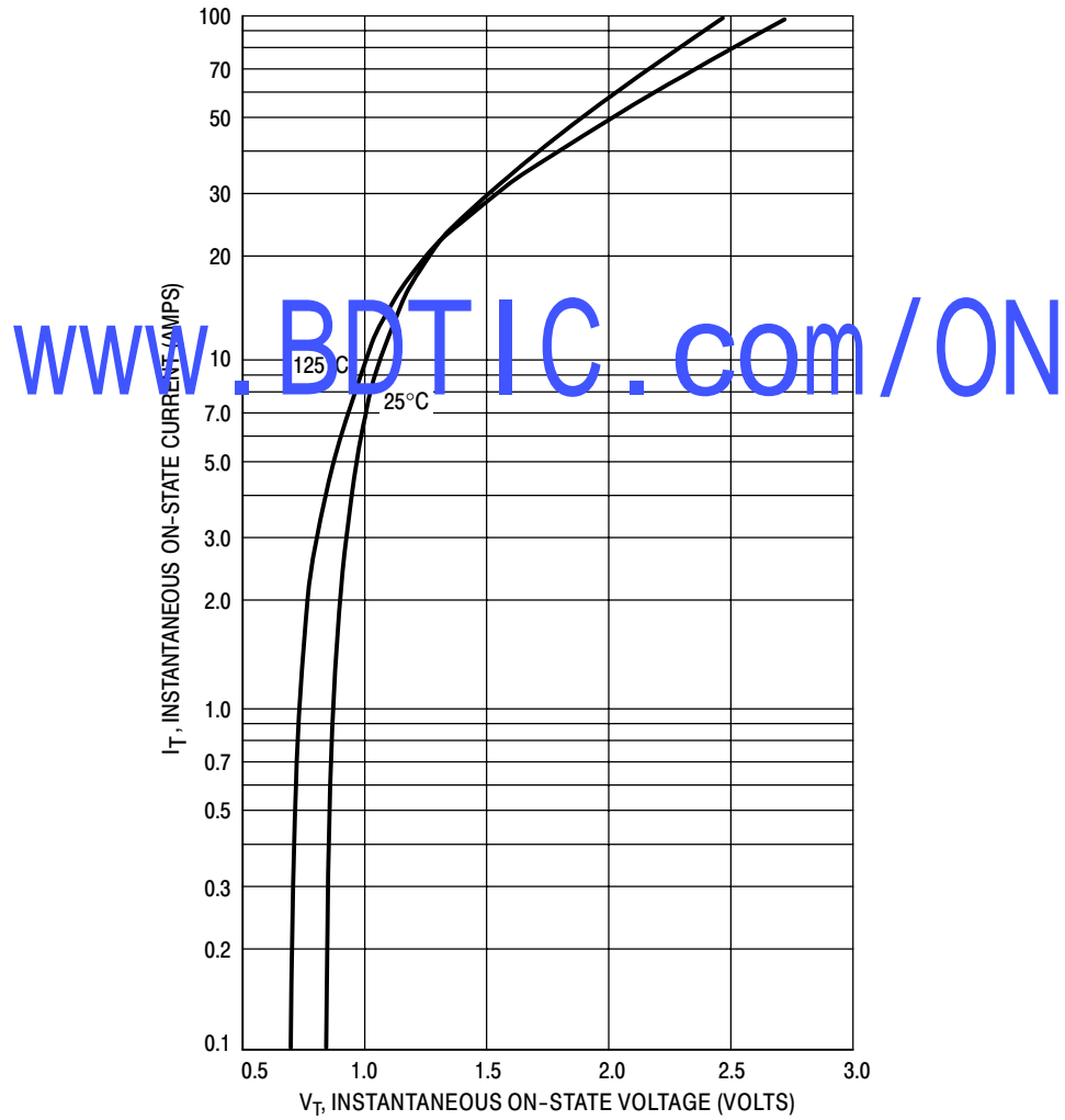
Figure 7. Typical On-State Characteristics
