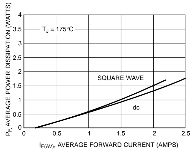
Figure 8. Power Dissipation
