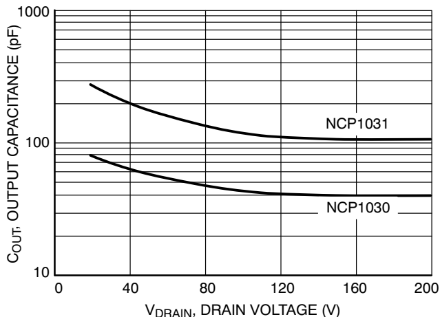
Figure 22. Power Switch Circuit Output Capacitance vs. Drain Voltage
