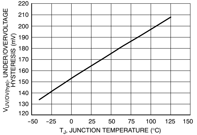
Figure 17. Line Under/Overvoltage Hysteresis vs. Junction Temperature
