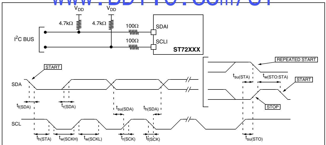
Figure 96. Typical Application with I 2 C Bus and Timing Diagram
