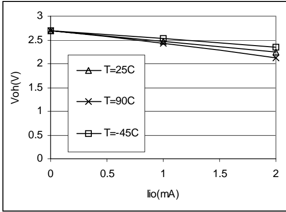
Figure 85. Typ. V_{OH} at V_{DD}=4V
