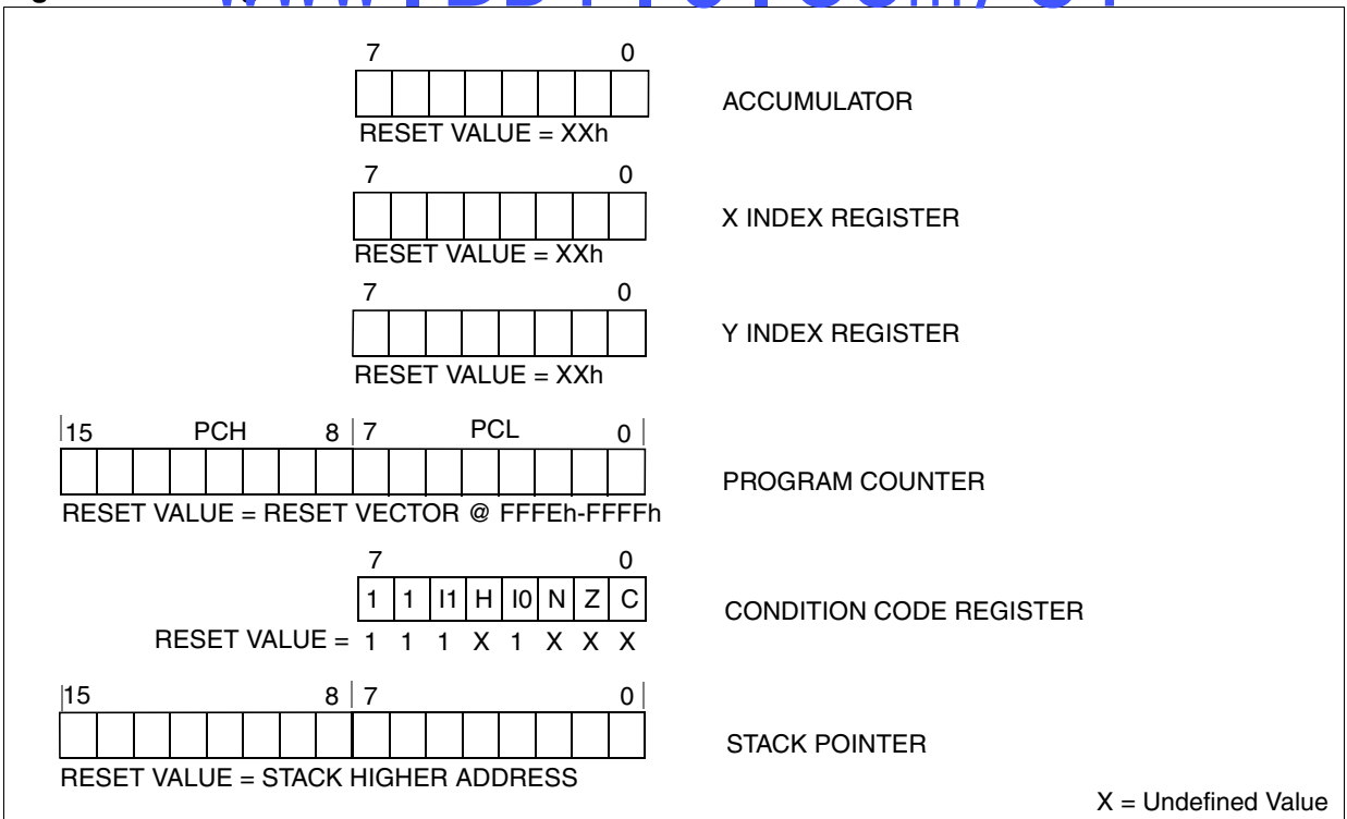
Figure 7. CPU Registers www.bdtic.com/ST
