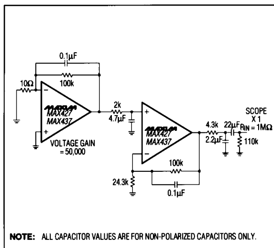
Figure 1. Voltage-Noise Test Circuit (0.1Hz to 10Hz)
