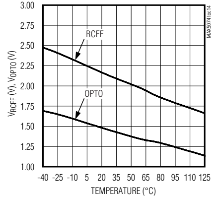
MINIMUM RCFF AND OPTO LEVELS vs. TEMPERATURE
