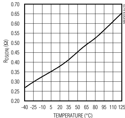
POWER MOSFETS Rps(ON) vs. TEMPERATURE
