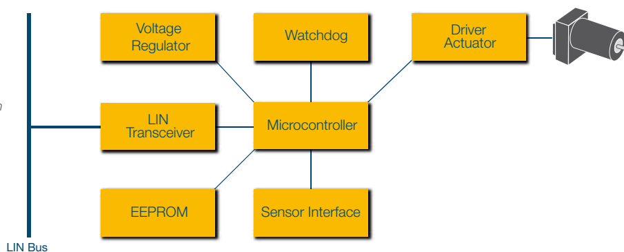
Intelligent partitioning: typical block schematic with LIN bus connection for a DC motor application
