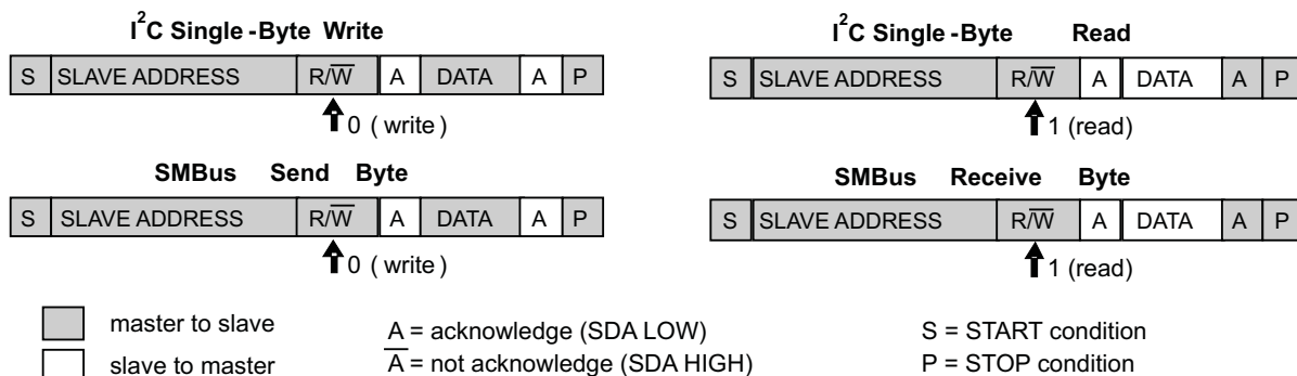
Figure 1. I 2 C Single-Byte Write and Read Compared to SMBus Send and Receive Byte
