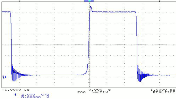
Full Load Switching
