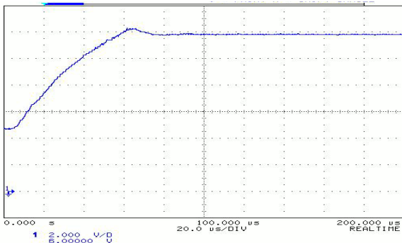
Start Up from Enable into Full Load
