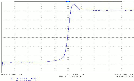
Switch Full Load Rise Time
