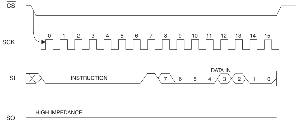
Figure 4-5. WRSR Timing
