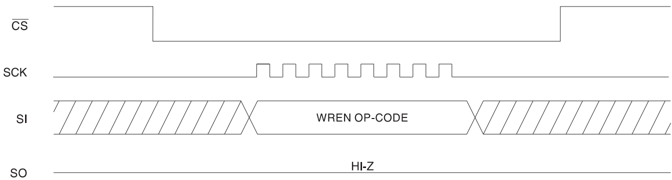
Figure 4-3. WRDI Timing
