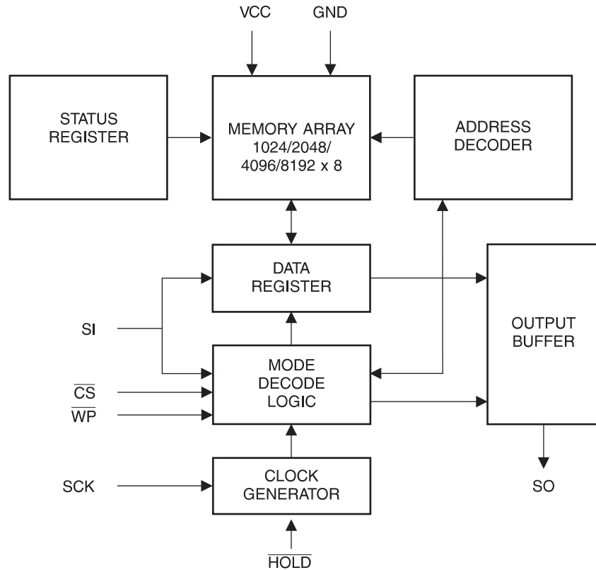
Figure 1-1. Block Diagram
