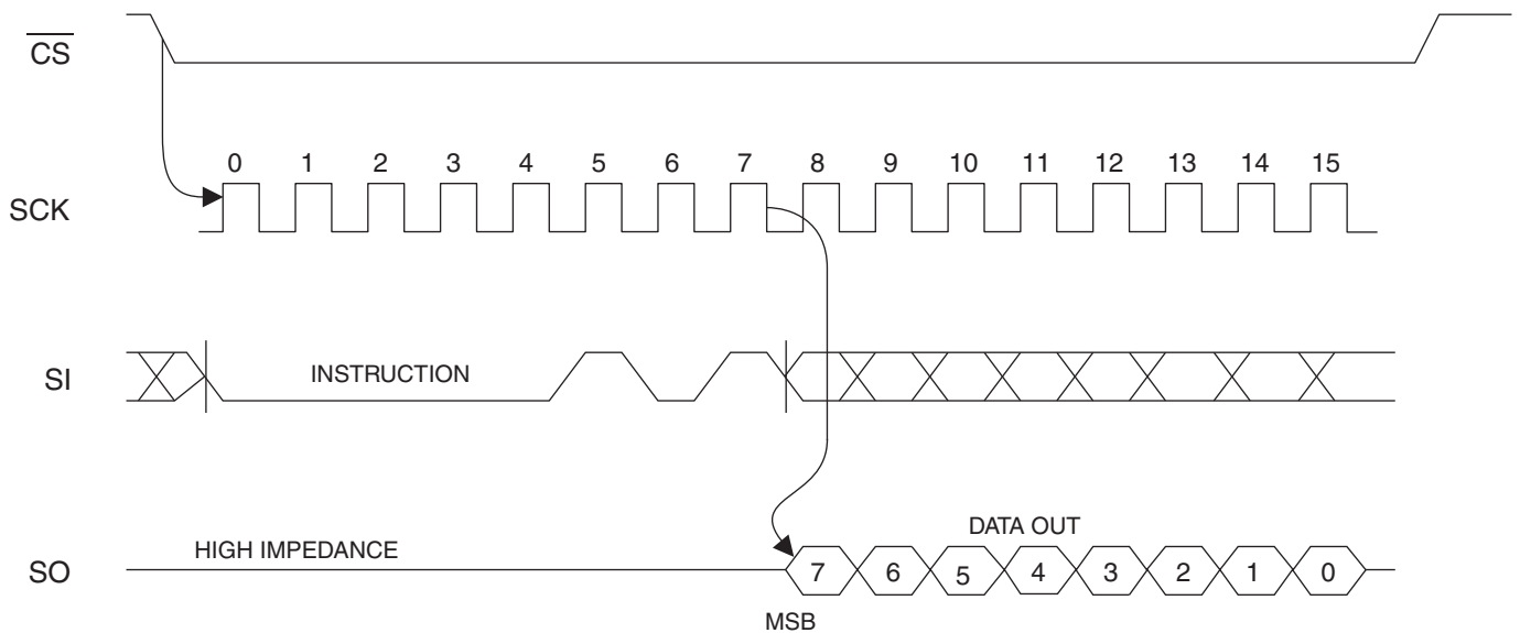
Figure 4-4. RDSR Timing
