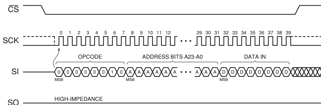
Figure 8-1. Byte Program
