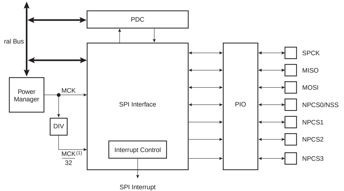
Figure 23-1. Block Diagram
