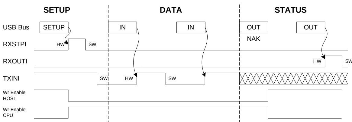
Figure 30-16. Control Read
