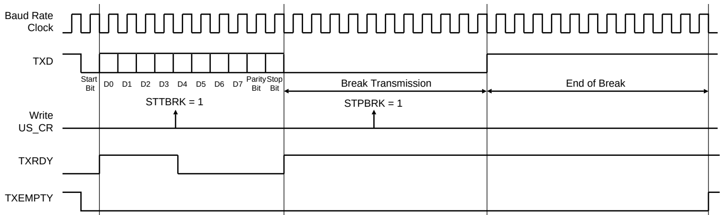
Figure 26-26. Break Transmission
