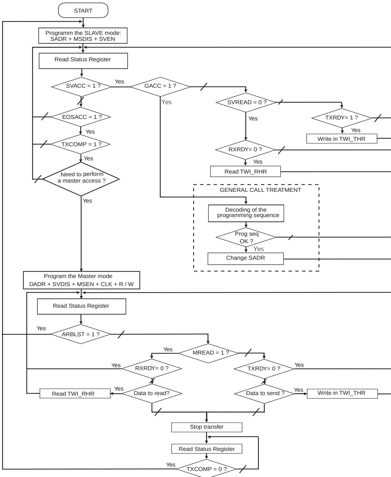
Figure 24-21. Multi-master Flowchart
