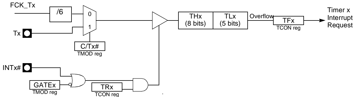
Figure 90. Timer/Counter x (x= 0 or 1) in Mode 0
