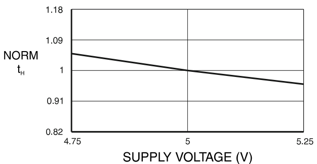
NORMALIZED t_H VS. SUPPLY VOLTAGE (TA = 25°C)
