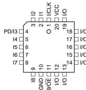
PLCC
