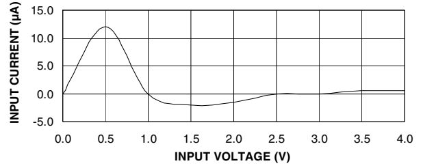
ATF22LV10CZ/CQZ INPUT CURRENT VS. INPUT VOLTAGE ( V_{CC} = 3.3V , T_A = 25^\circ C )
