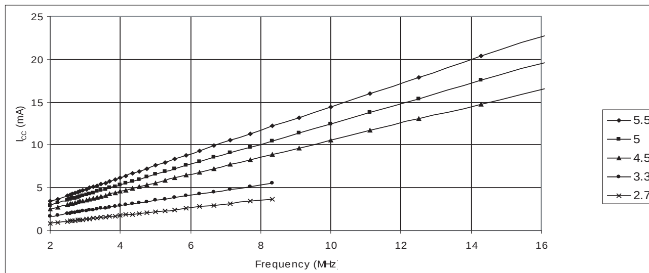
Figure 31-12. Active Supply Current vs Frequency, T=25°C
