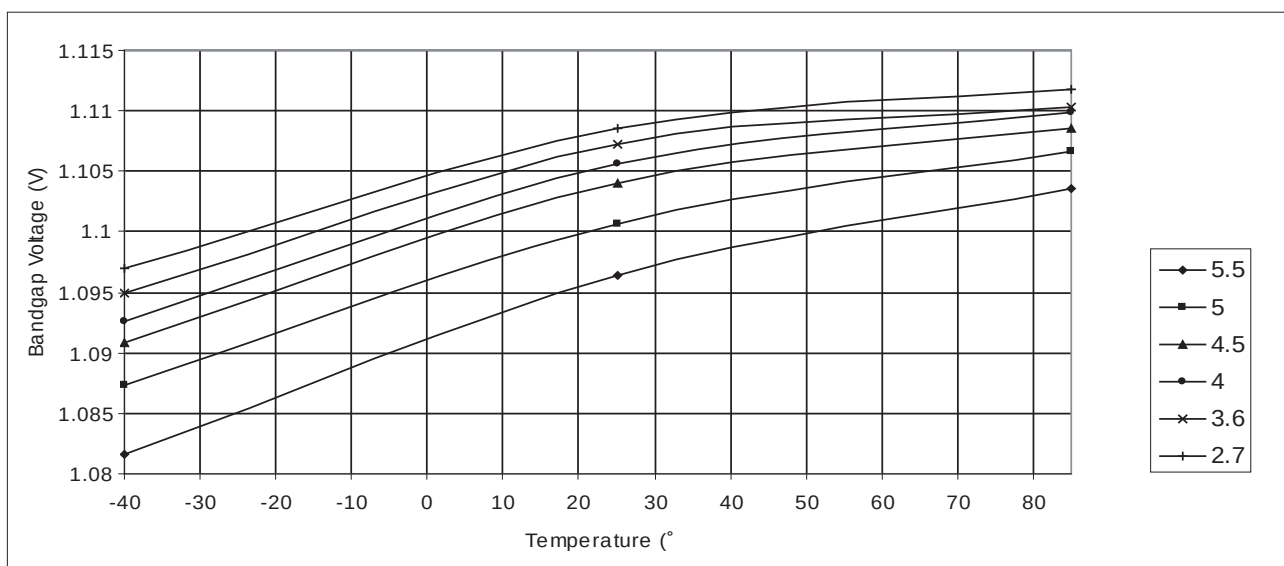
Figure 31-16. Bandgap voltage vs. Temperature
