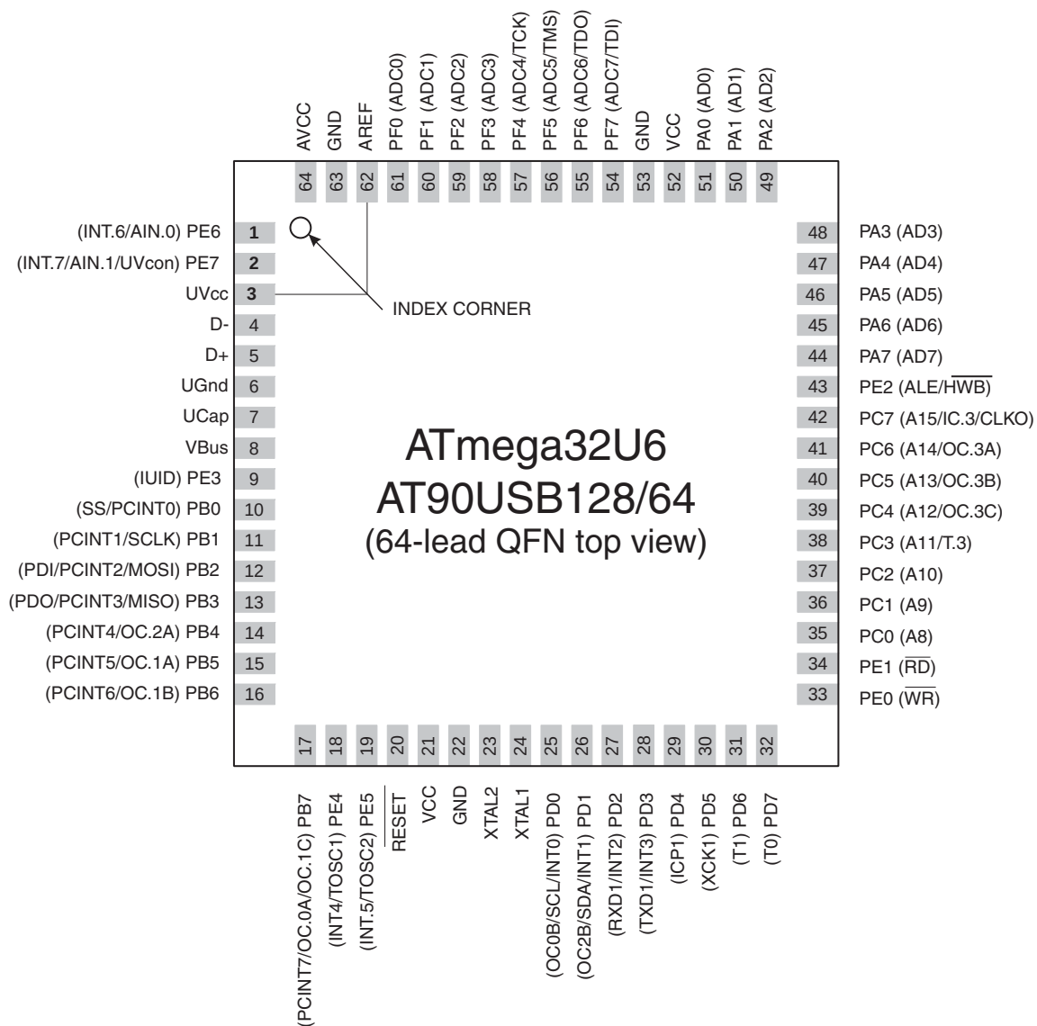
Figure 1-2. Pinout ATmega32U6/AT90USB64/128-QFN
