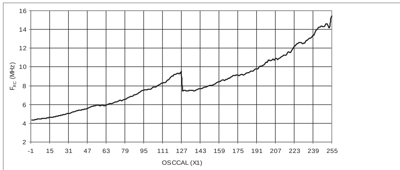
Figure 31-24. RC Oscillator Frequency vs. OSCCAL, T=25°C
