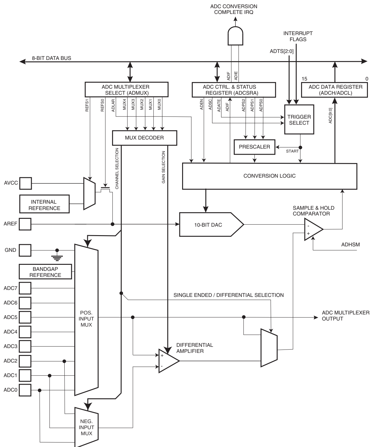
Figure 25-1. Analog to Digital Converter Block Schematic
