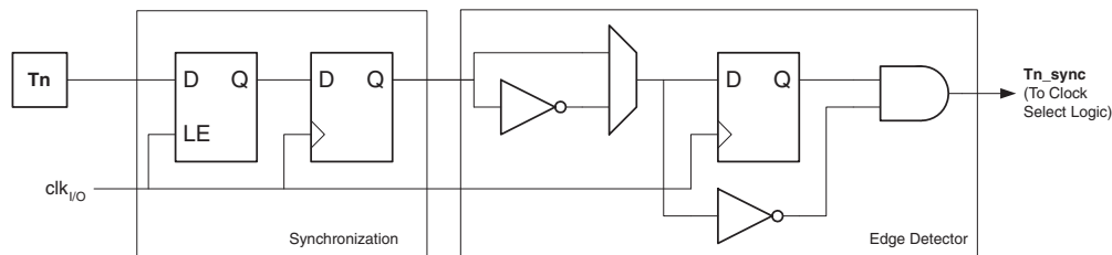
Figure 1. Tn/T0 Pin Sampling
