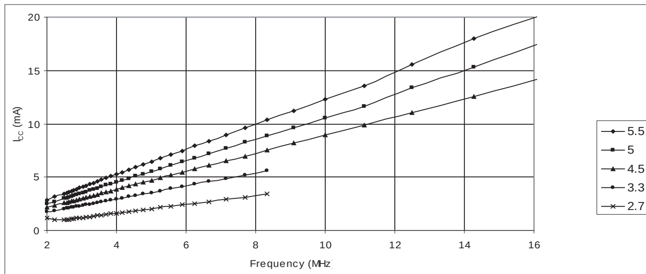
Figure 31-11. Idle Supply Current vs Frequency, T=25°C
