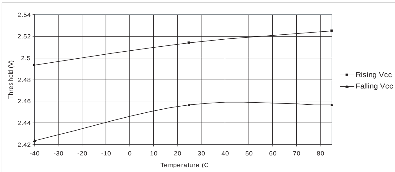
Figure 31-20. BOD Voltage (2.4V level) vs. Temperature
