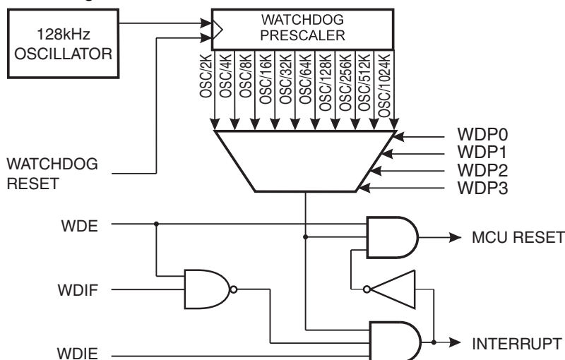
Figure 8-7. Watchdog Timer
