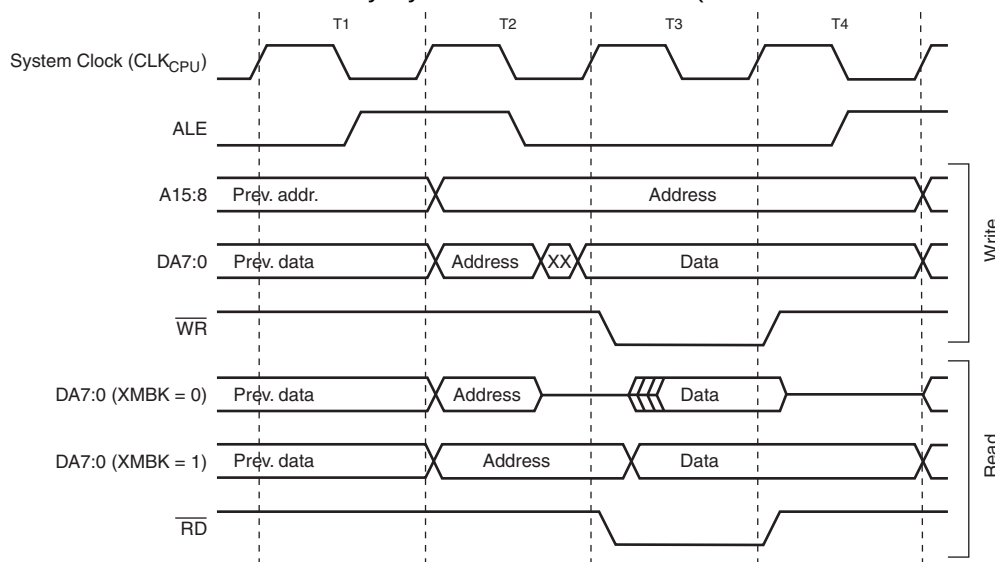
Figure 5-6. External Data Memory Cycles without Wait-state (SRWn1=0 and SRWn0=0)
