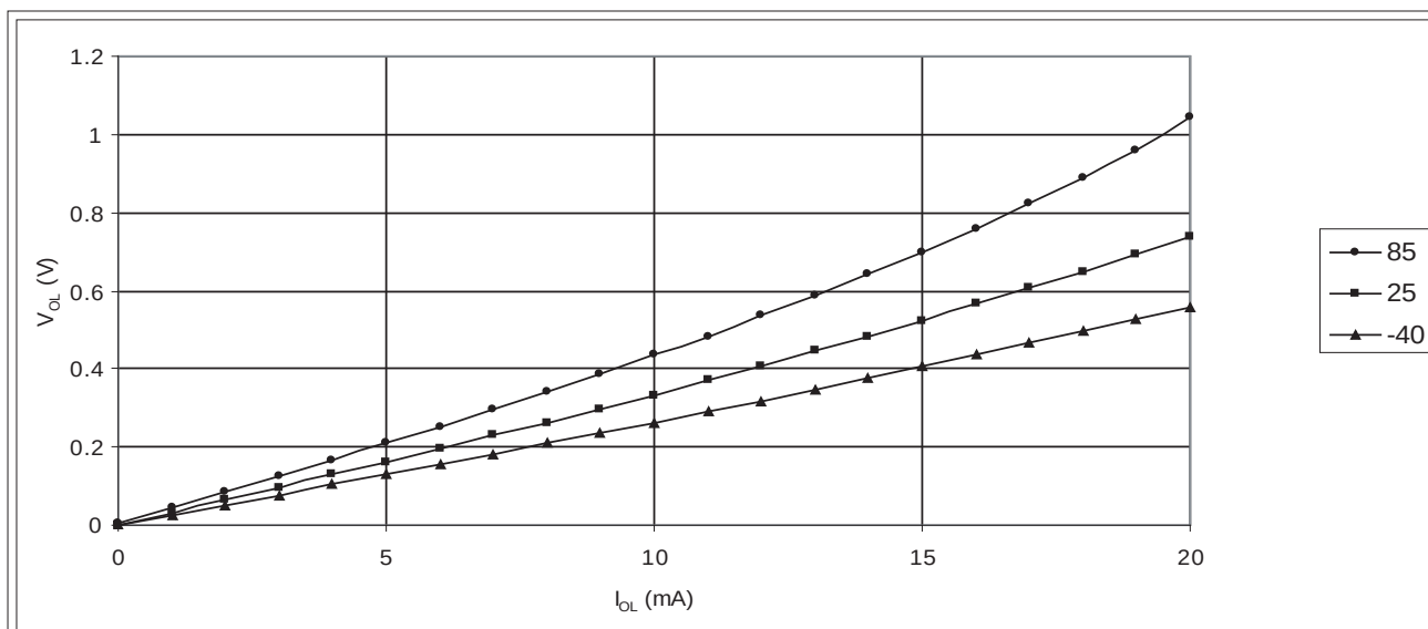
Figure 31-3. Output Low Voltage vs. Output Current, all I/Os excluding DP/DM, V_{CC}=3V
