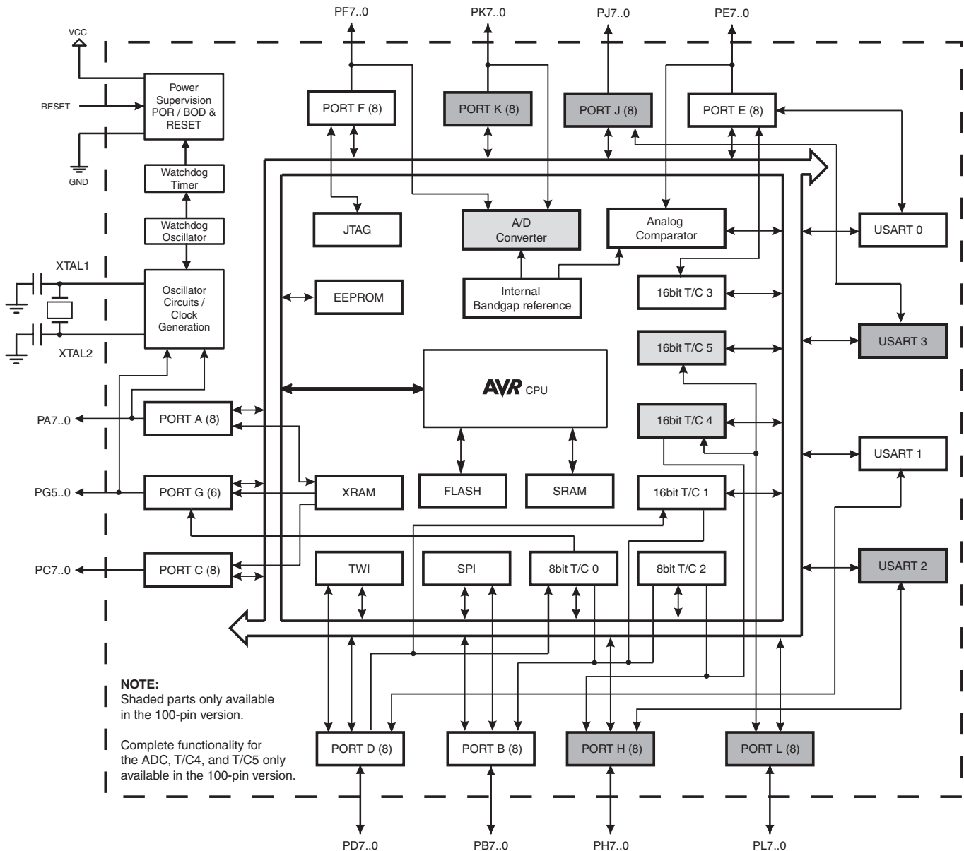
Figure 3-1. Block Diagram
