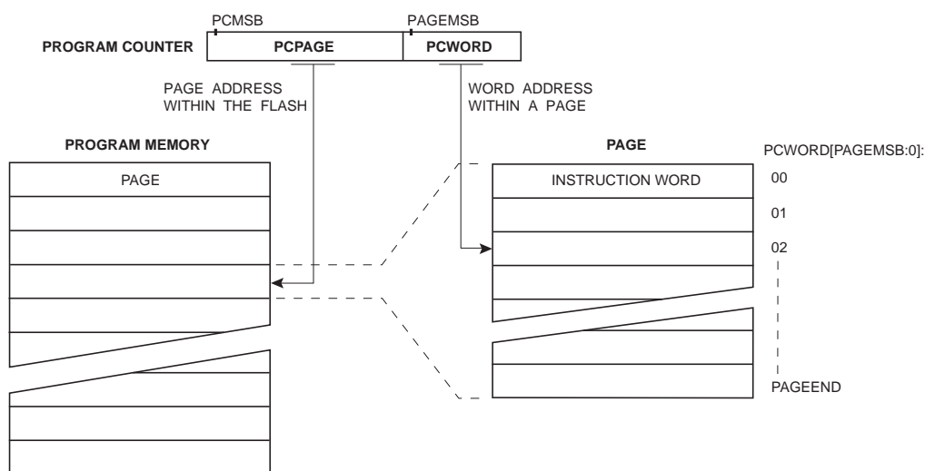
Figure 21-2. Addressing the Flash Which is Organized in Pages
