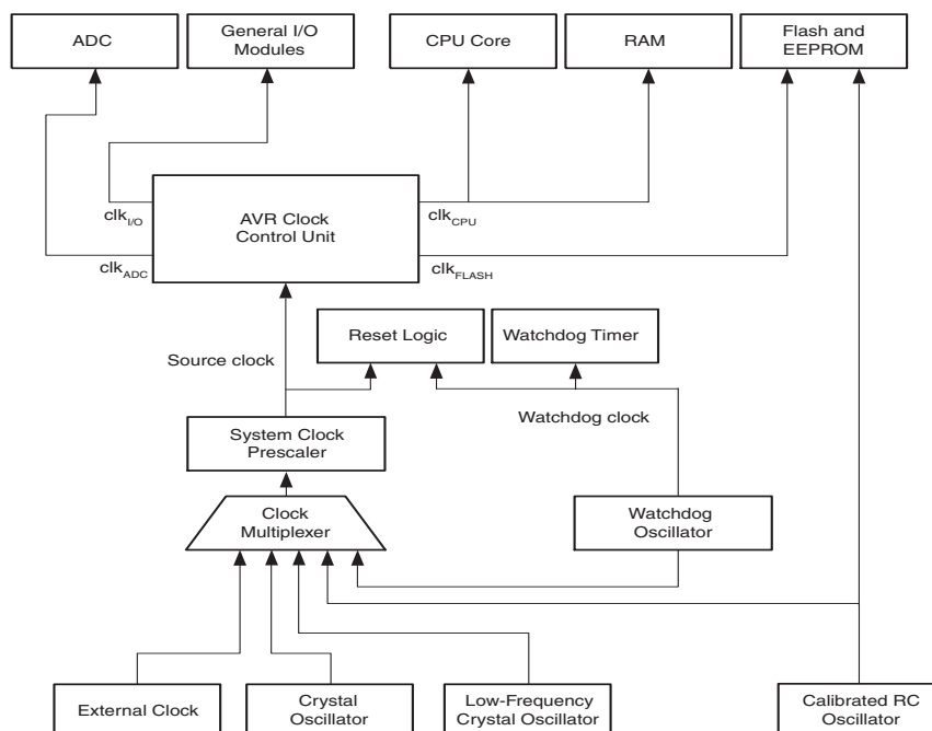
Figure 7-1. Clock Distribution
