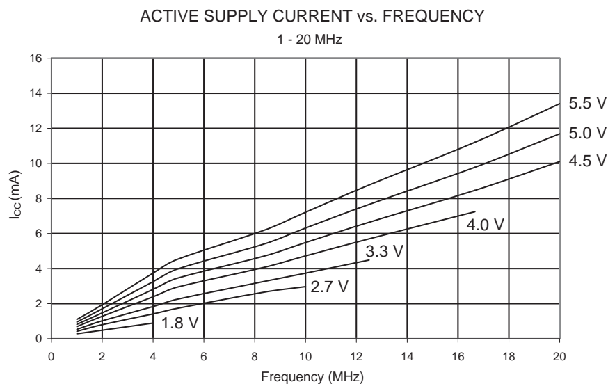
Figure 24-2. Active Supply Current vs. Frequency (1 - 16 MHz)
