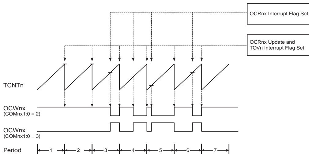
Figure 16-11. Fast PWM Mode, Timing Diagram
