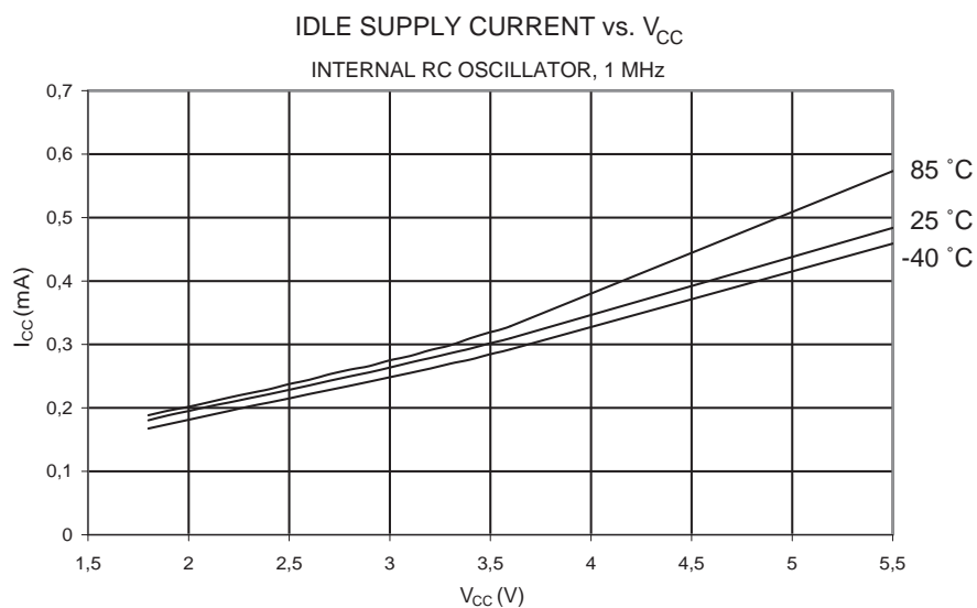
Figure 24-9. Idle Supply Current vs. V_{CC} (Internal RC Oscillator, 1 MHz)
