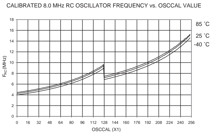
Figure 24-33. Calibrated 8.0 MHz RC Oscillator Frequency vs. OSCCAL Value
