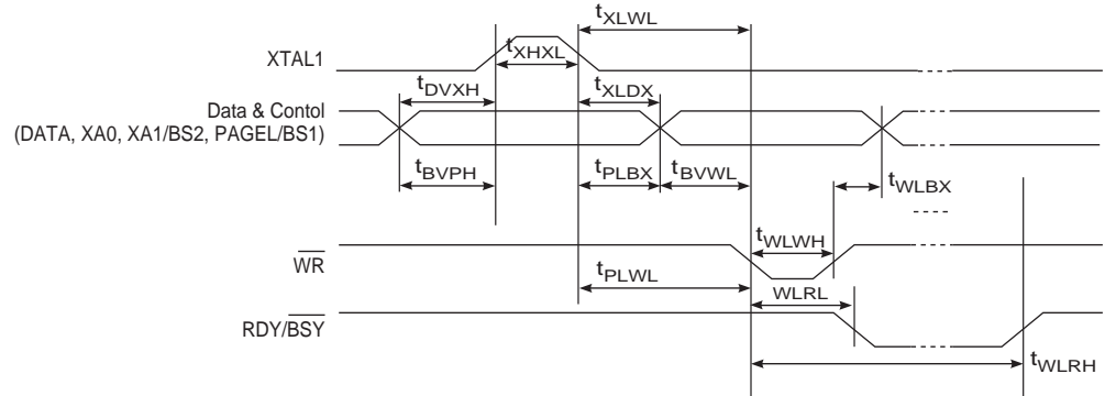
Figure 23-3. Parallel Programming Timing, Including some General Timing Requirements
