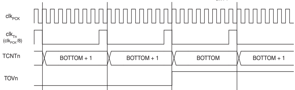
Figure 16-17. Timer/Counter Timing Diagram, with Prescaler ( f_{clkT1}/8 )
