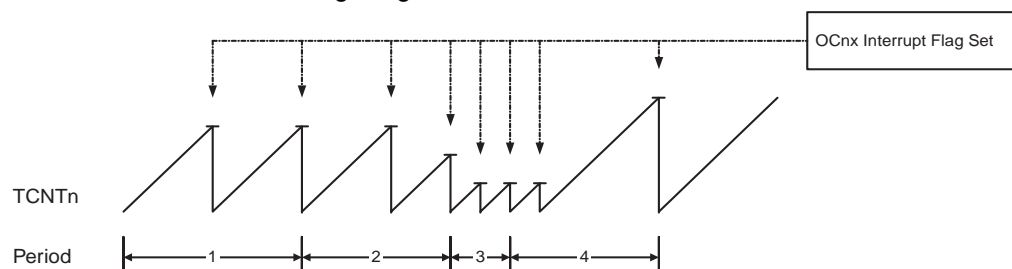
Figure 14-2. CTC Mode, Timing Diagram
