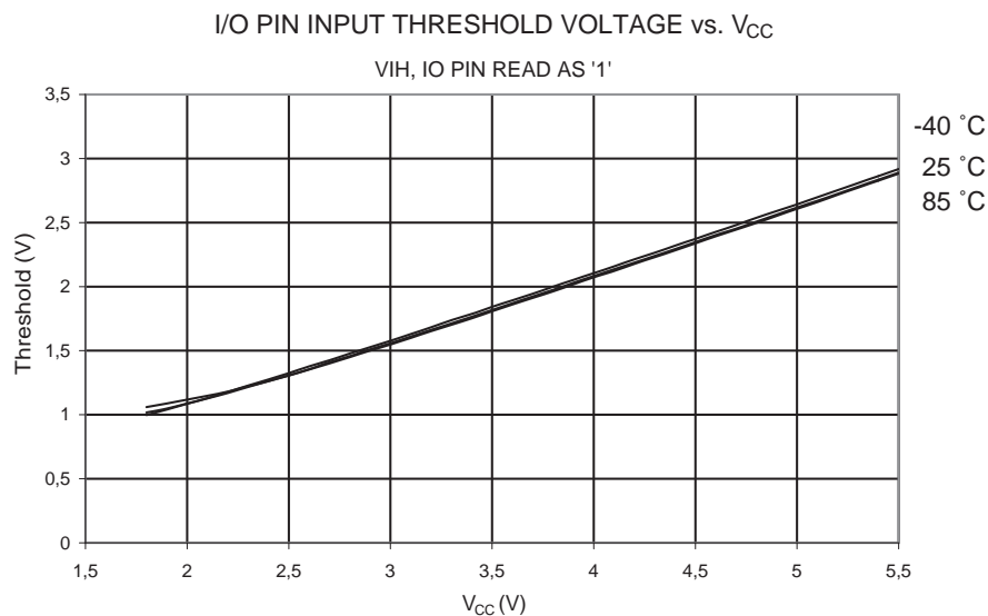
Figure 24-21. I/O Pin Input Threshold Voltage vs. V_{CC} ( V_{IH} , I/O Pin Read as '1')
