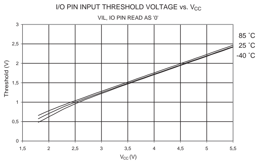
Figure 24-22. I/O Pin Input Threshold Voltage vs. V_{CC} ( V_{IL} , I/O Pin Read as '0')
