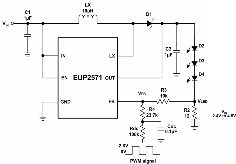
Figure 7. Filtered PWM Signal for LED Dimming Control
